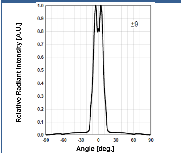
Radiation Characteristics
